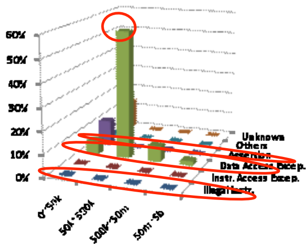
Linux System
