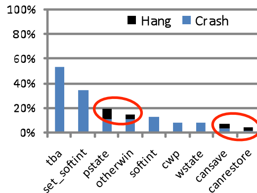
Solaris System
