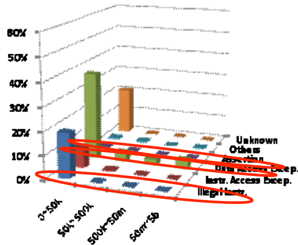
Solaris System
