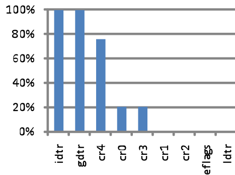
Linux System
