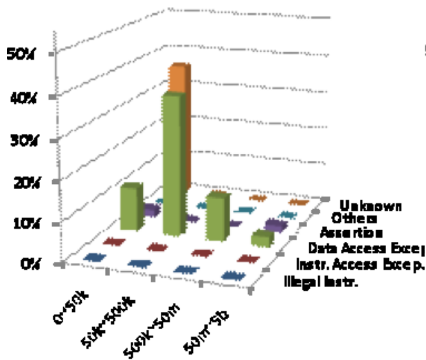
Linux System
